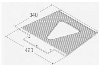
Toe plate G - 420 x 340 x 7 mm Accessory 930.003
