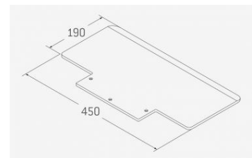
Toe plate DS-NG - 450 x 190 x 7 mm Accessory 930.085
