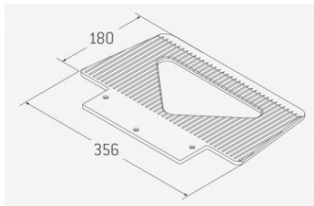
Toe plate WL - 356 x 180 x 7 mm Accessory 930.018
