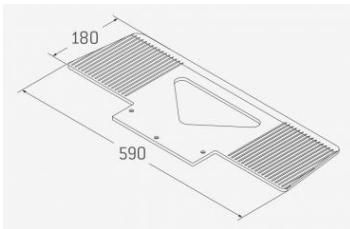
Toe plate XWL - 590 x 180 x 7 mm Accessory 930.074
