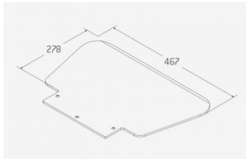
Toe plate LH - 467 x 278 x 5 mm Accessory 930.002
