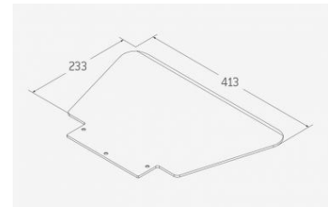
Toe plate V - 413 x 233 x 5 mm Accessory 930.001
