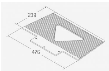
Toe plate GS - 476 x 240 x 7 mm Accessory 930.030
