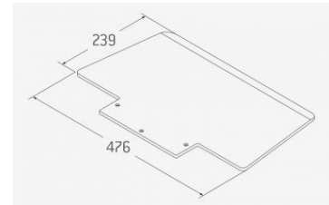
Toe plate GS-NG - 476 x 240 x 7 mm Accessory 930.084
