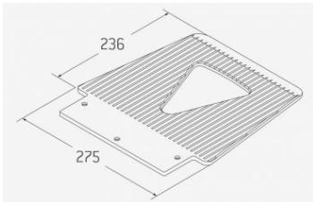
Toe plate Standard - 275 x 236 x 7mm Accessory 030.025
